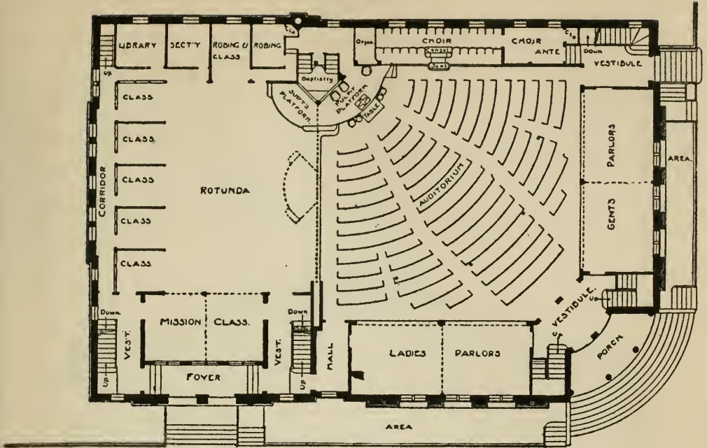
MAIN FLOOR FIRST CHRISTIAN CHURCH, ATHENS, GA.
